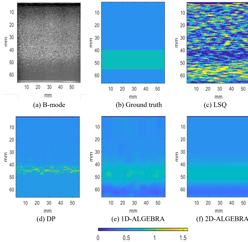
Fig. 5. Parametric images of the local attenuation (computed from Eq. (30)) of phantom C (attenuation step). The color bar shows the value of local attenuation.
