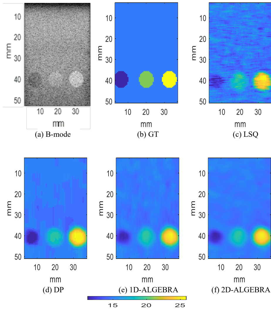
Fig. 8. Parametric image of the backscatter coefficient at the center frequency of phantom E (inclusion phantom). Results are shown on a dB scale with respect to 10^{-4} \text{ cm}^{-1} \text{ sr}^{-1} .
