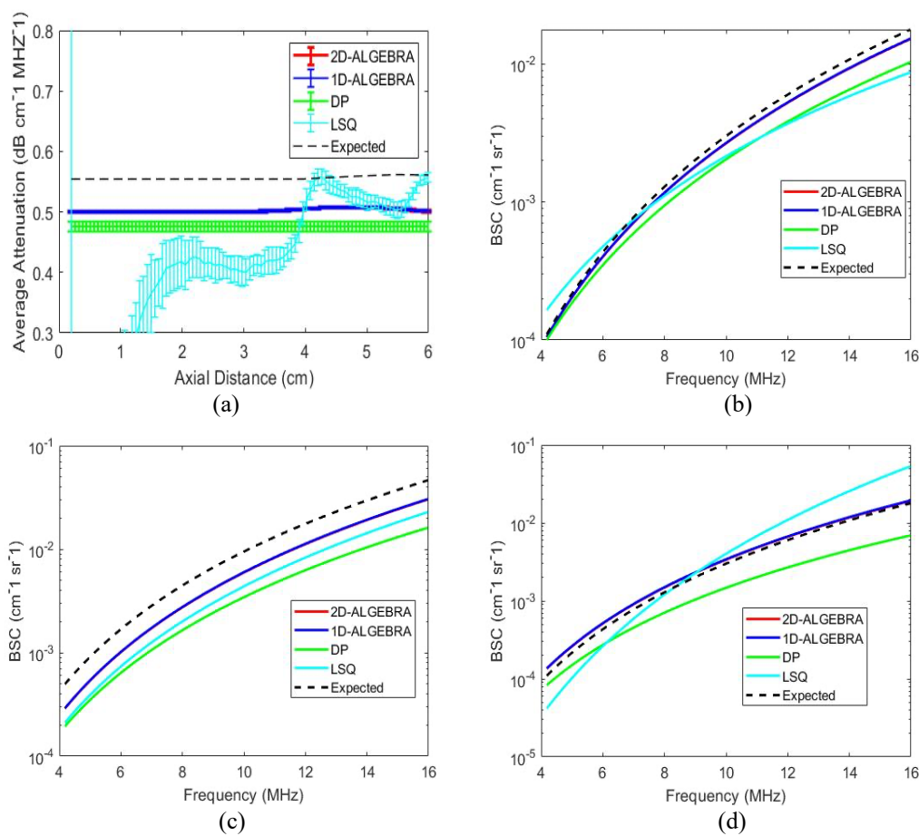
Fig. 6. Results of 1D-ALGEBRA (blue), 2D-ALGEBRA (red), DP (green), and LSQ (cyan) in phantom D (backscatter step). The error bars show the standard deviation over the 860 samples for the effective attenuation (a) and reconstructed BSC averaged over 400 samples in layer 1 (b), layer 2 (c), layer 3 (d). The black dashed line is the expected value. The red curve is superimposed by the blue curve.
