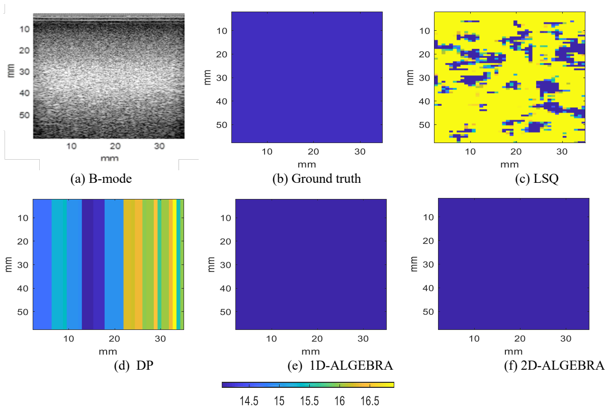
Fig. 3. Parametric images of the BSC at the center frequency in phantom A (uniform). Results are shown on a dB scale with respect to 10^{-4} \text{ cm}^{-1} \text{ sr}^{-1} . The colorbar shows BSC at the center frequency.
