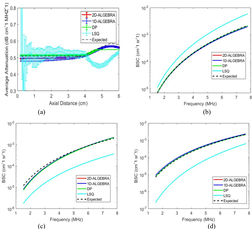
Fig. 4. Results of 1D-ALGEBRA (blue), 2D-ALGEBRA (red), DP (green), and LSQ (cyan) in phantom C (attenuation step). The error bars show the standard deviation over the 860 samples for attenuation coefficient (a) and reconstructed BSC averaged over 400 samples in layer 1 (b), layer 2 (c), layer 3 (d). The black dashed line is the ground truth values. The red curve is superimposed by the blue curve.
