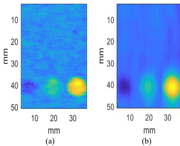
Fig. 9. Influence of regularization weights in the parametric images of phantom E with 1D-ALGEBRA. Weights in (a): [10 10 10], weights in (b): [ 10^4 10^4 10^4 ].
